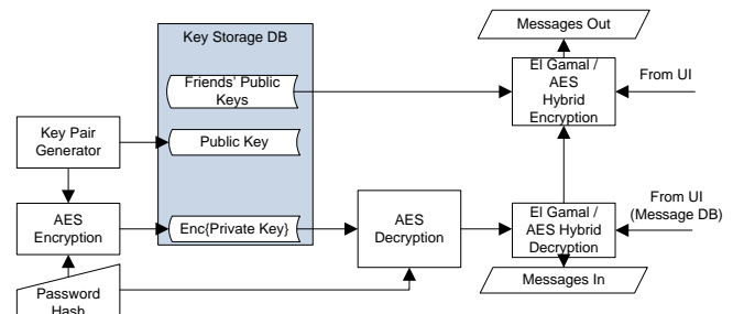
Figure 2. flyByNight Architecture.
