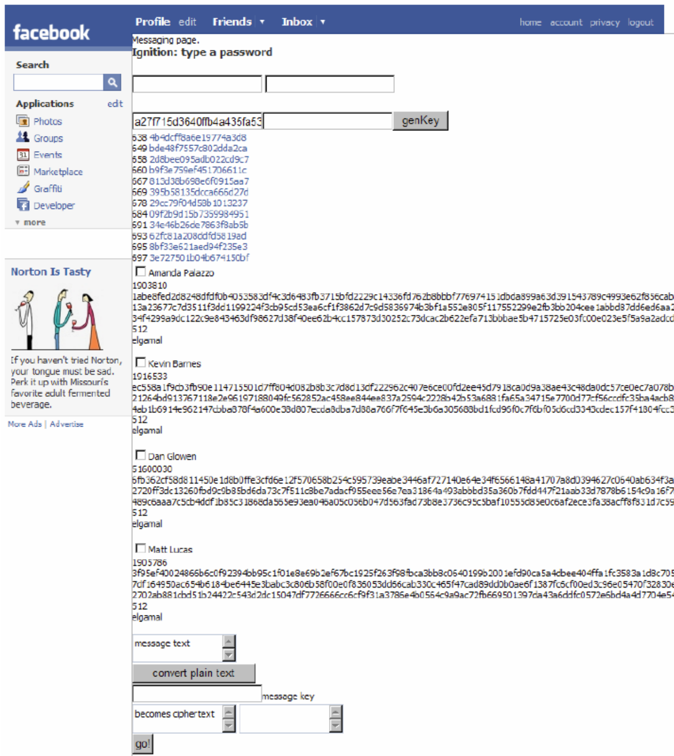
Figure 3. flyByNight Facebook Application. To send a message, the user checks the boxes corresponding to the intended recipients of the message, types the message text, and clicks “go!” A list of the messages a user has received, indexed by the first blocks of their ciphertexts, appear at the top; to read one of these, the user types his password and clicks the ciphertext block. The plaintext then appears in a dialog box.
