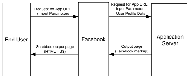
Figure 1. Facebook Application dataflow.
